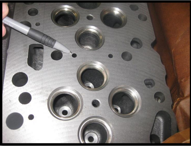
Above: 6.7L, 24V, COMMON RAIL, 2007.5 & UP, There are 2 steam vent holes between each of the cylinders.
